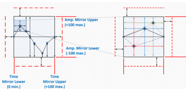
Figure 3. A schematic representation of GENDYN timbre synthesis geometry showing one cycle of a wave-form within boundary limits, followed by a single magnified vertex with an imagined displacement. The movement of this vertex (indeed all vertices of the waveform), follows a random walk that is influenced by a probability distribution function selected by the user.
