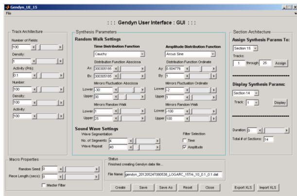
Figure 6. The GENDYN user interface as implemented in the Matlab programming environment.
