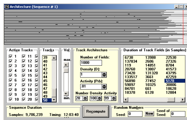
Figure 4. The track architecture dialogue of the New GENDYN Program user interface shown with the maximum number of 50 tracks of sound. This is one section of a GENDYN construction. There are potentially 50 separate sections that can be generated by the program, each with as many as 50 tracks.
