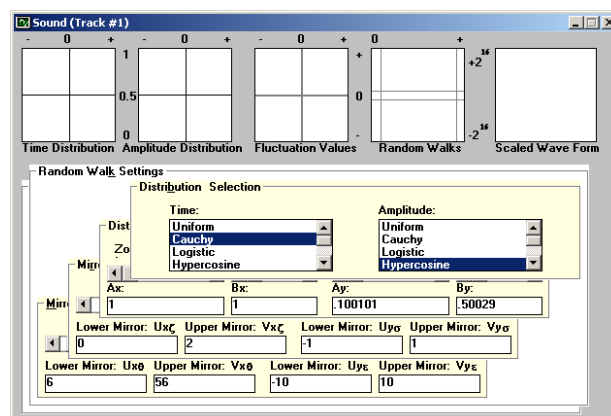
Figure 5. The timbre sound synthesis dialogue window of the New GENDYN Program.
